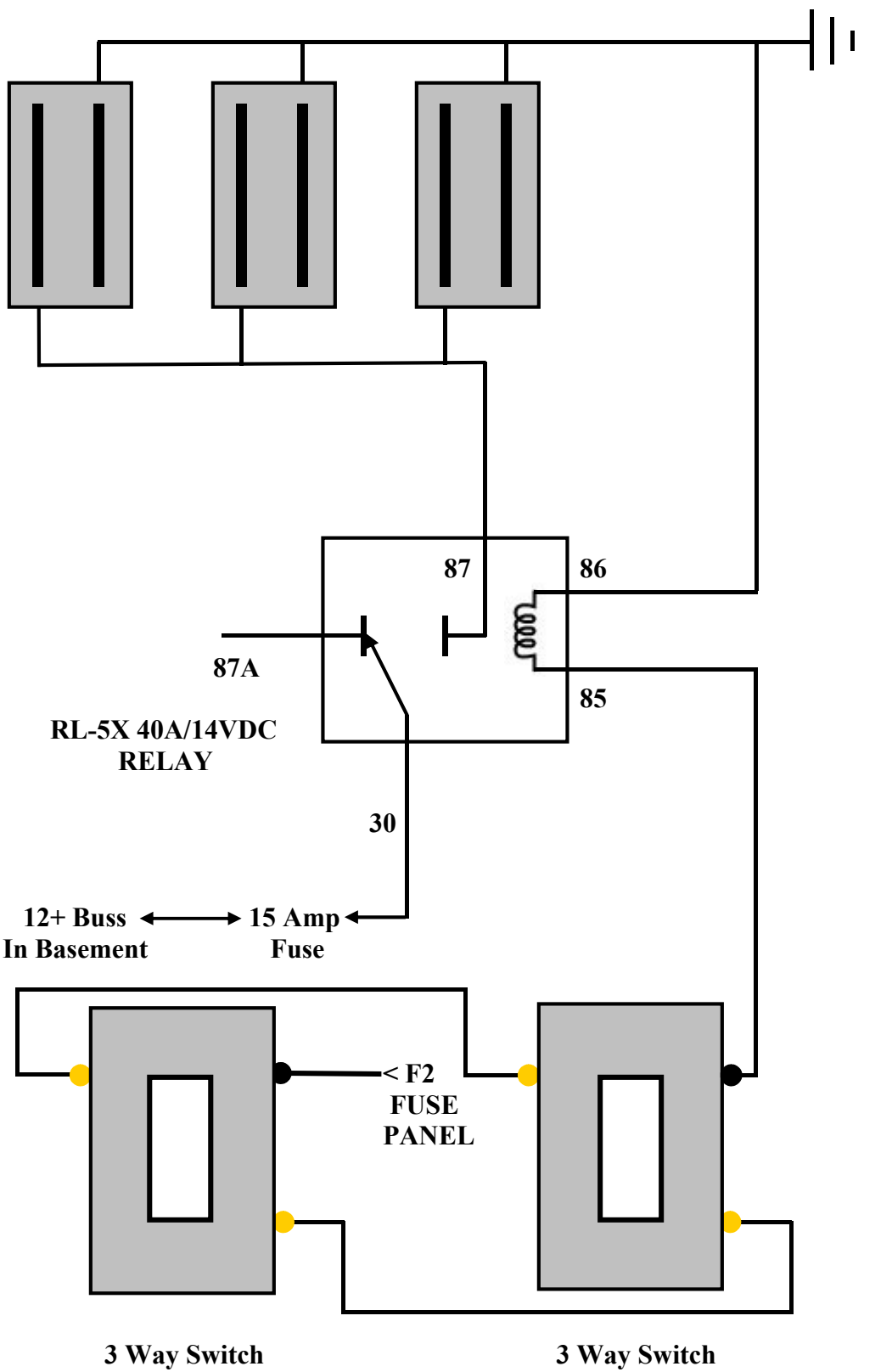
3 Way Switching for Living Room Fluorescent Lighting
